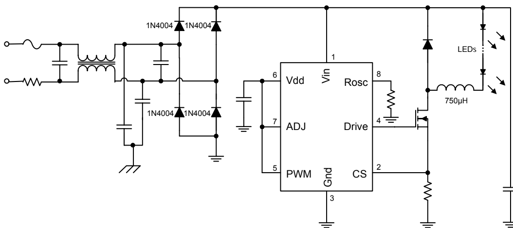
Figure 5 Buck Driver
